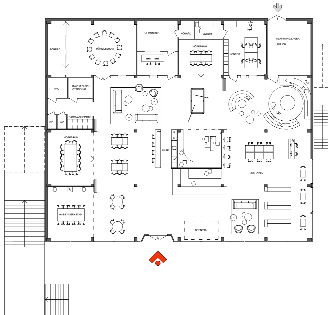
PLAN 0, NEDRE TORGET 1:200 (A3)
