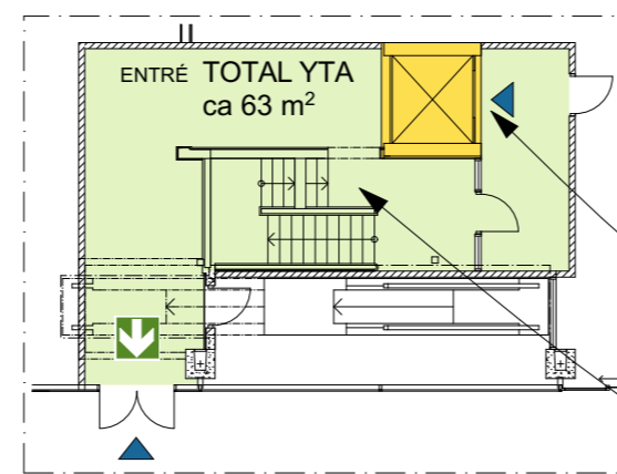
PLAN 3 - GATUPLAN
