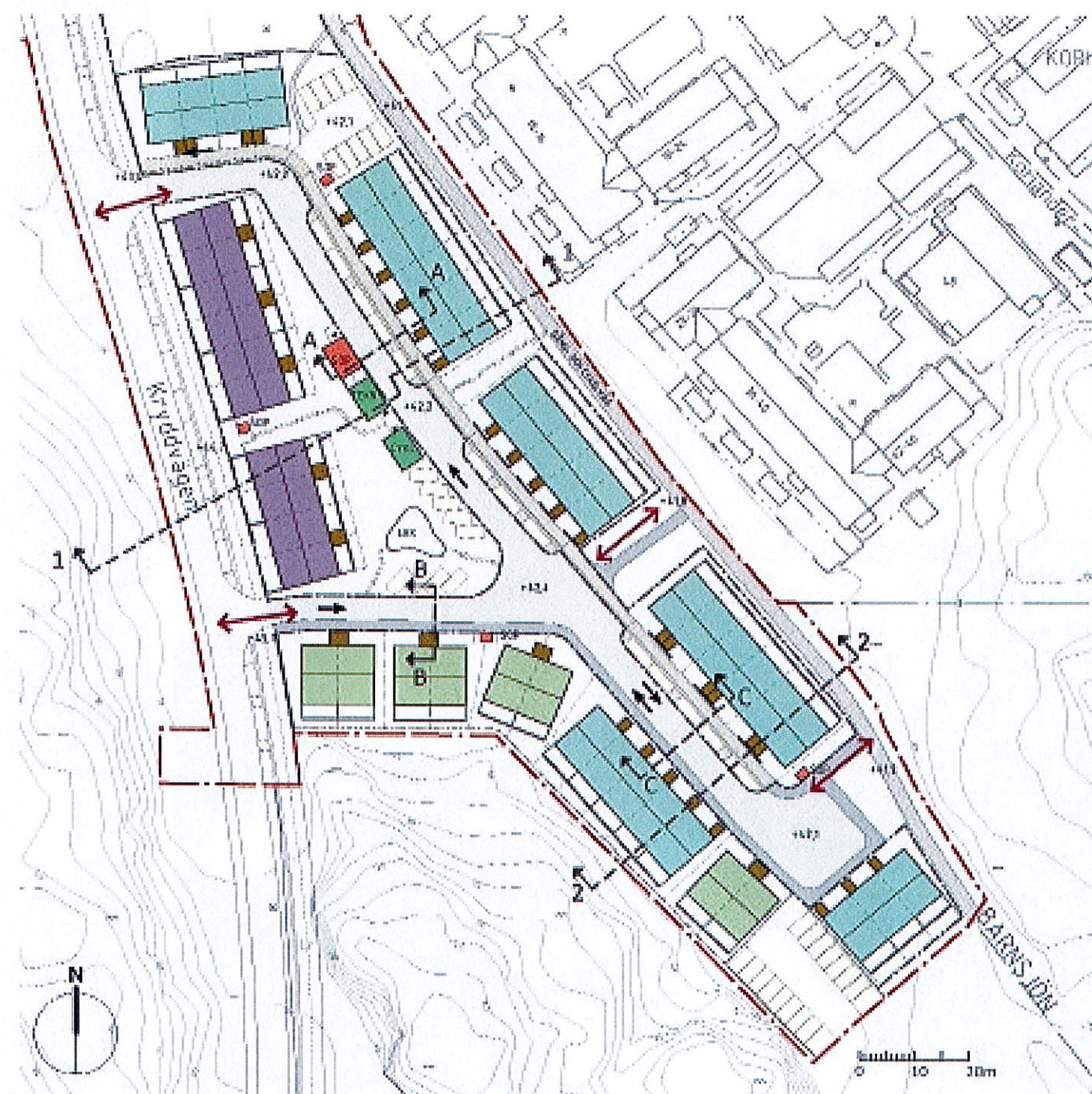
Situationsplan
