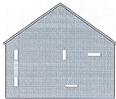
Gavel, fasadskiss
