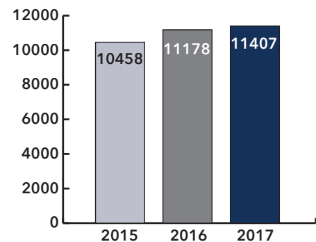
Diagram 5. Antal larm 2015-2017.
