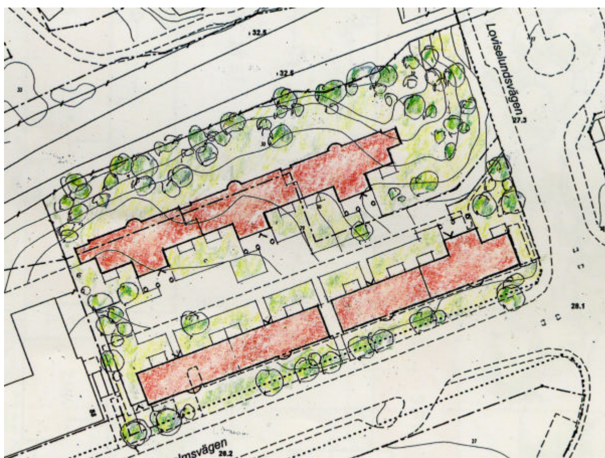
Situationsplan
